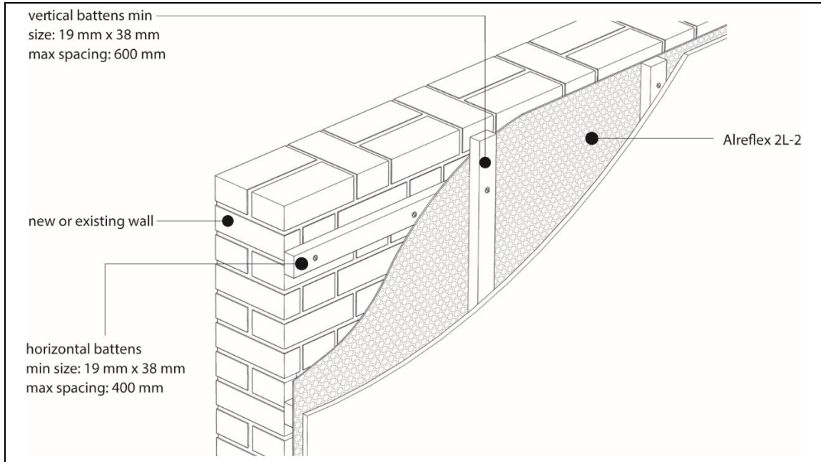
Figure 1 General arrangement
