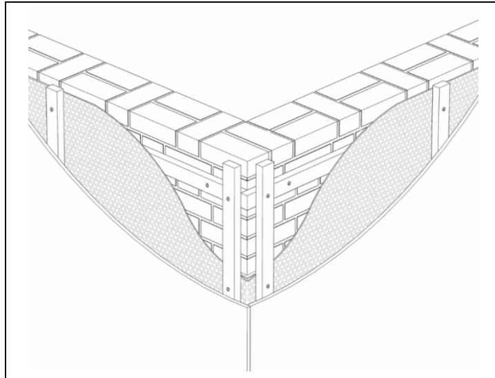
Figure 3 Typical external corner detail
