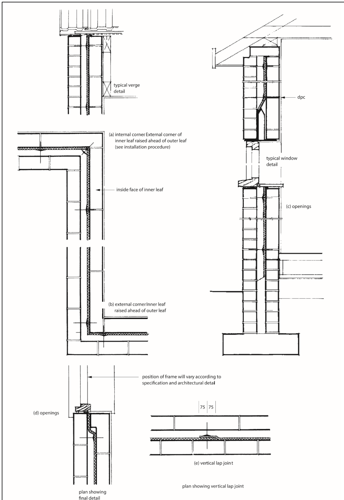
Figure 4 Fixing details (dimensions in mm)
