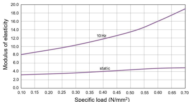
Vibration isolation
