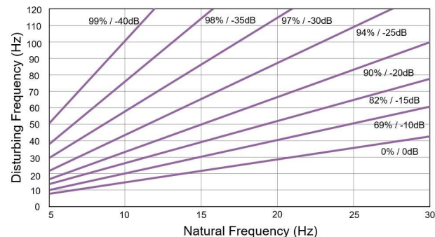
Vibration isolation
