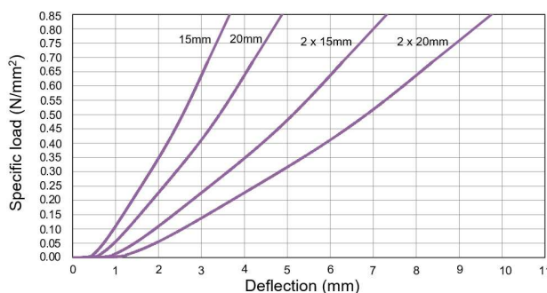
Load deflection curve
