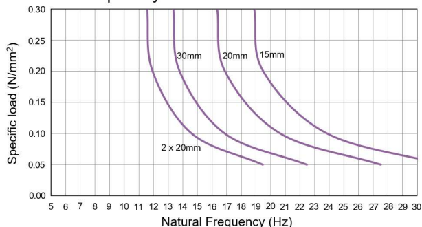
Natural frequency
