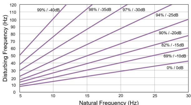
Vibration isolation
