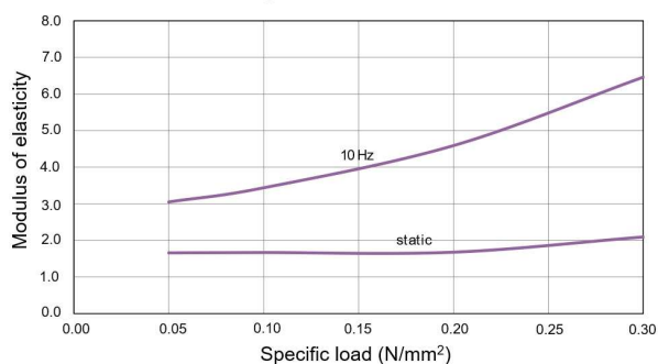
Modulus of elasticity
