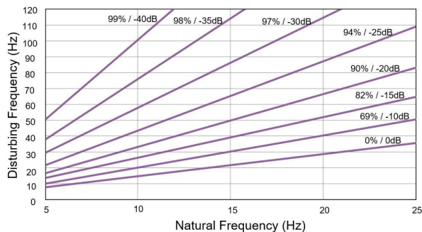
Vibration isolation
