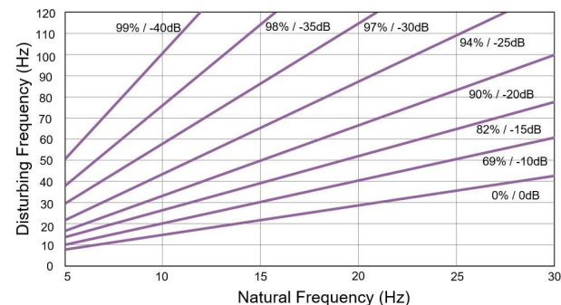
Vibration isolation
