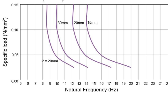
Natural frequency
