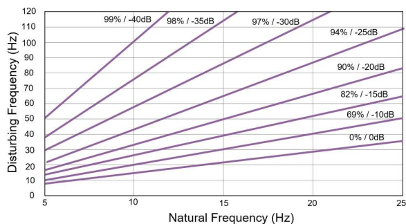
Vibration isolation
